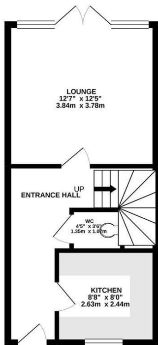
GROUND FLOOR 356 sq.ft. (33.1 sq.m.) approx.
